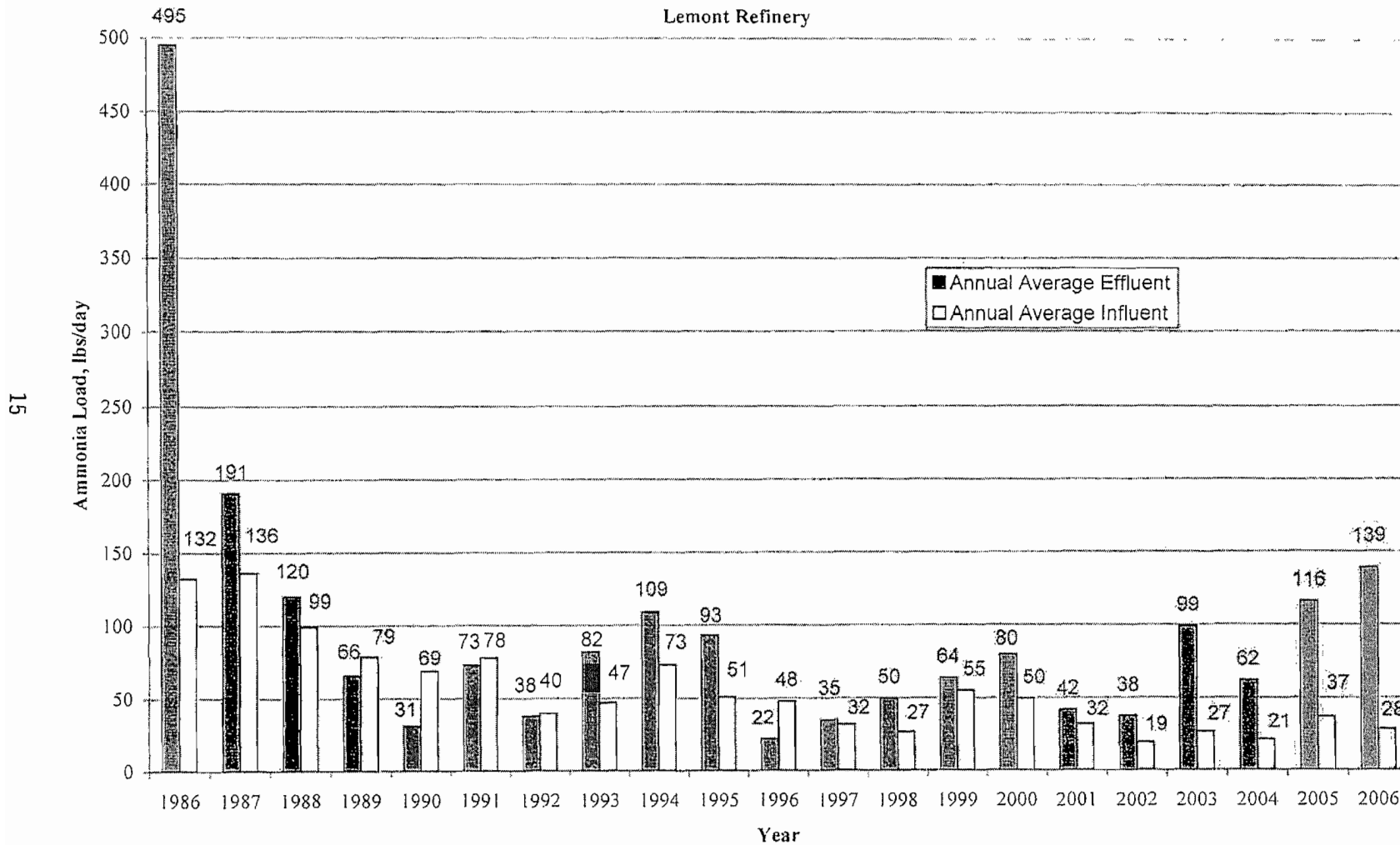
Figure 3-4 ANNUAL AVERAGE AMMONIA INFLUENT AND EFFLUENT LOADING Lemont Refinery
