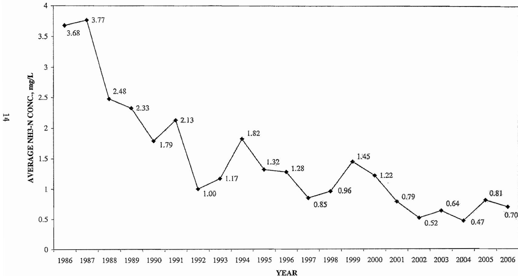
Figure 3-3 ANNUAL AVERAGE INFLUENT AMMONIA CONCENTRATION Sanitary & Ship Canal
