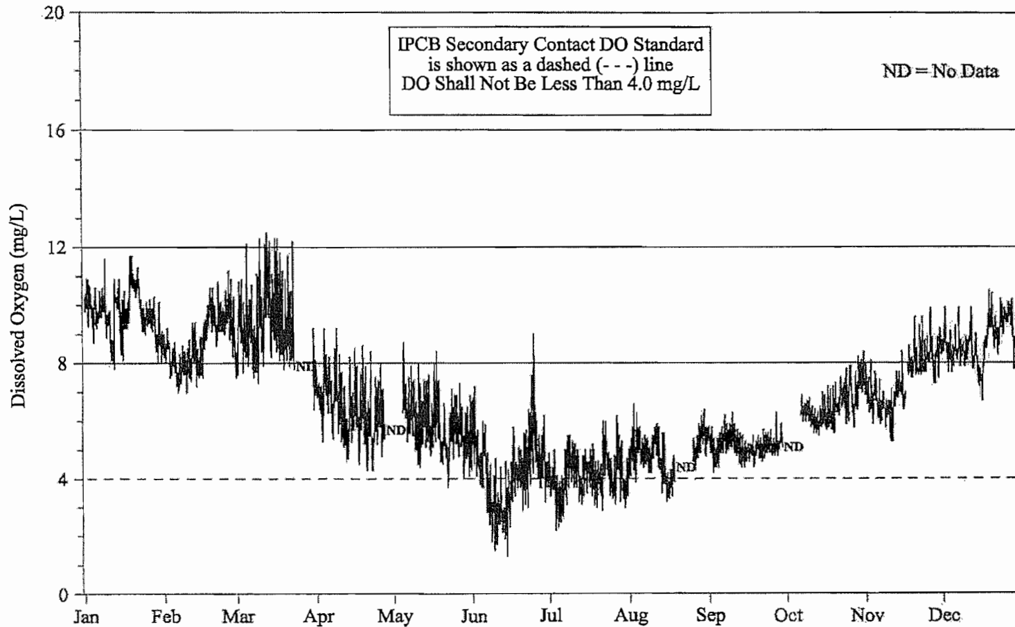
FIGURE 15: DISSOLVED OXYGEN CONCENTRATION MEASURED HOURLY AT JEFFERSON STREET ON THE DES PLAINES RIVER FROM JANUARY 2005 THROUGH DECEMBER 2005
