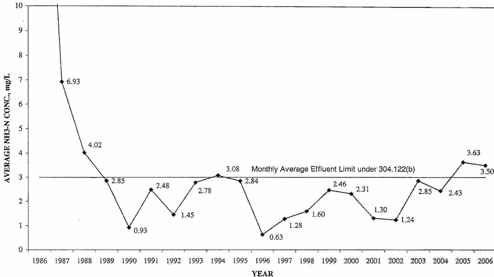
Figure 3-1 ANNUAL AVERAGE EFFLUENT AMMONIA CONCENTRATION Lemont Refinery
