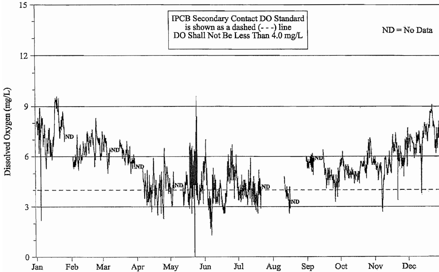
FIGURE 13: DISSOLVED OXYGEN CONCENTRATION MEASURED HOURLY AT ROUTE 83 ON THE CHICAGO SANITARY AND SHIP CANAL FROM JANUARY 2005 THROUGH DECEMBER 2005
